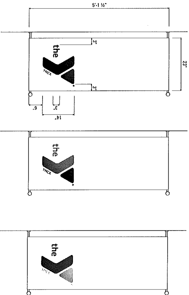
VERTICAL BANNER ELEVATION 3/4" = 1'-0"
