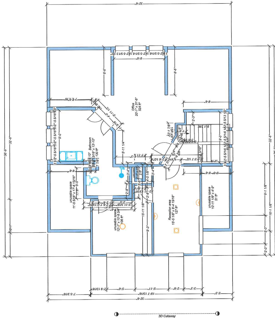
1309 S. Onieda St. 3rd. floor 830 sq. ft. Scale 1/8" = 1'
