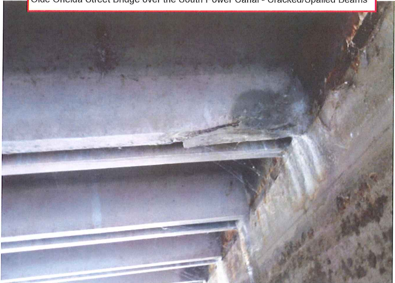
Olde Oneida Street Bridge over the South Power Canal - Cracked/Spalled Beams
