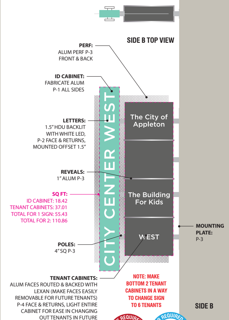
A DETAIL VIEWS 4 SCALE: 1/4" = 1'
